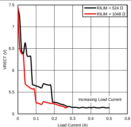
Figure 5. V_{RECT} vs I_{LOAD} at R_{LIM} = 524\ \Omega and 1048\ \Omega
