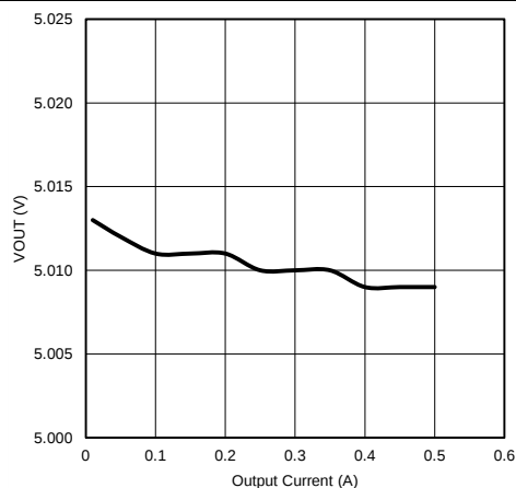
Figure 6. I_{LOAD} Sweep (I-V Curve)
