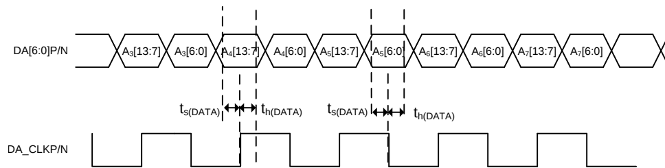
Figure 3. DAC3171 Input Data Timing Diagram for 7-Bit Interface Mode
