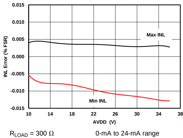
Figure 28. IOUT INL vs Supply (External R_{SET} )
