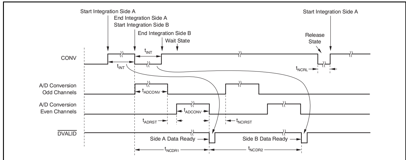
Figure 13. Conversion Detail for the Internal Operation of Noncontinuous Mode with Side A Integrated First
