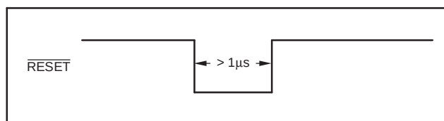
Figure 9. Reset Timing
