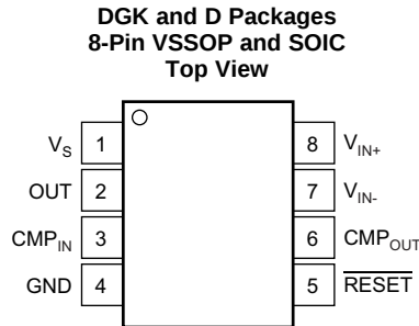
Pin Functions
