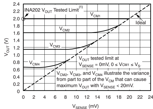
Figure 32. Example For Low V_{SENSE} Case 2 (INA202, Gain = 100)
