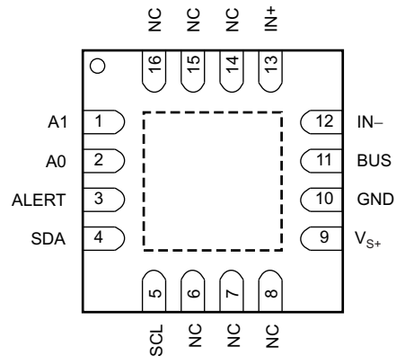
RGT PACKAGE QFN-16 (TOP VIEW)
