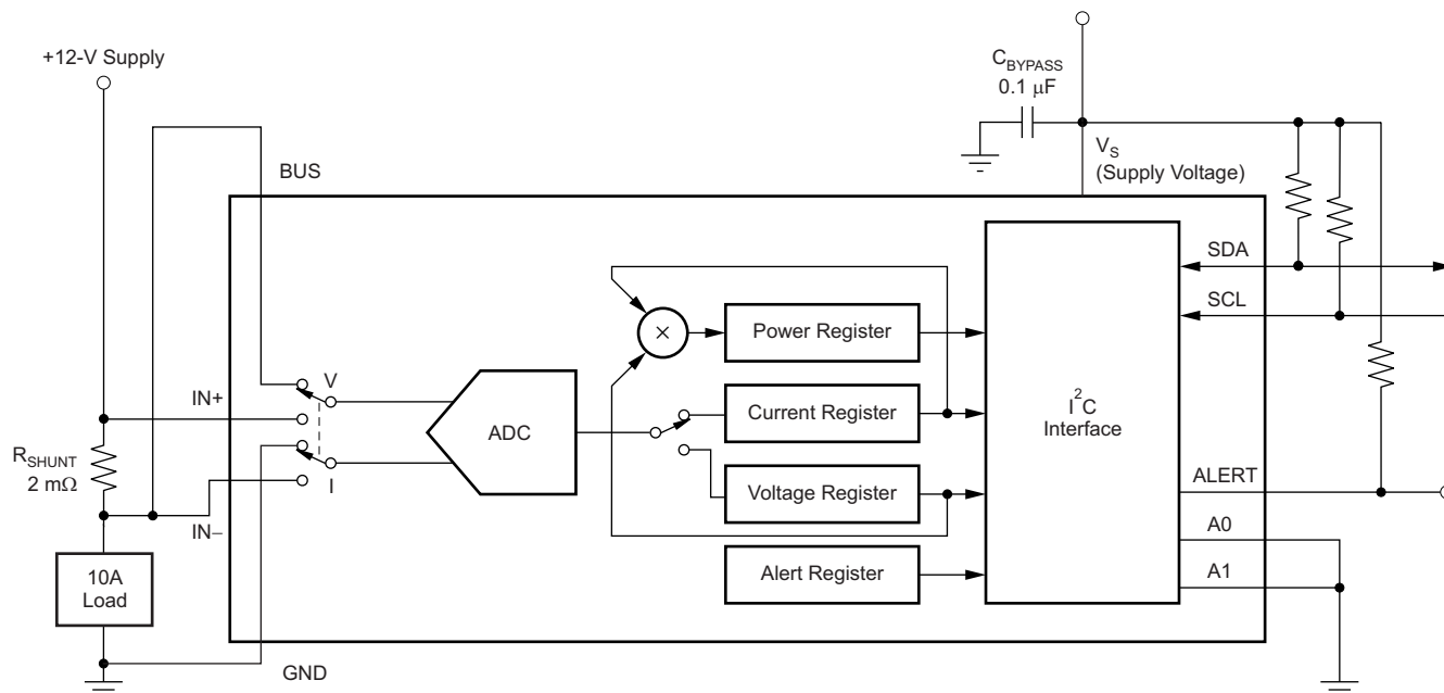
Figure 23. Example Circuit Configuration
