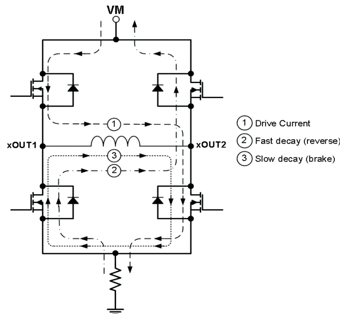
Figure 7. Decay Mode
