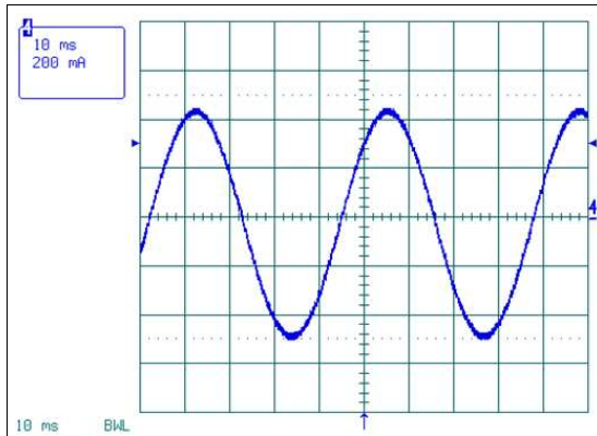
Figure 13. Microstepping Waveform, Phase A, Adaptive Decay
