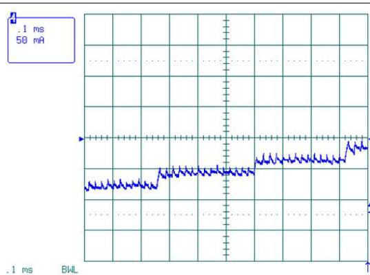
Figure 14. Microstepping Waveform, Adaptive Decay, Step Current Regulation
