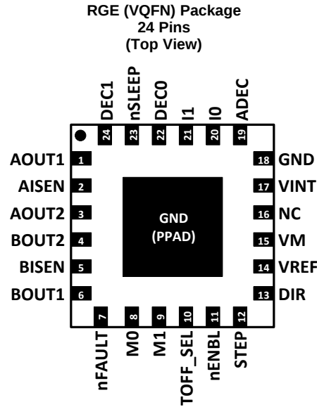
Pin Functions
