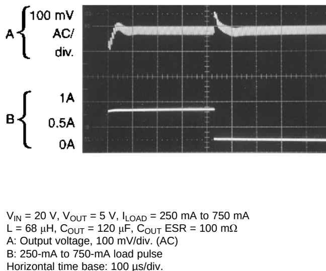
Figure 34. Load Transient Response for Continuous Mode
