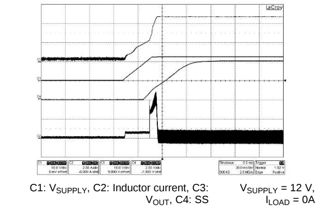
Figure 47. Start-Up
