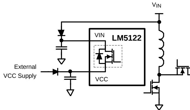
Figure 19. VIN Configuration when V_{IN} < V_{VCC}
