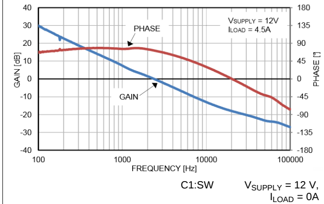
Figure 46. Loop Response
