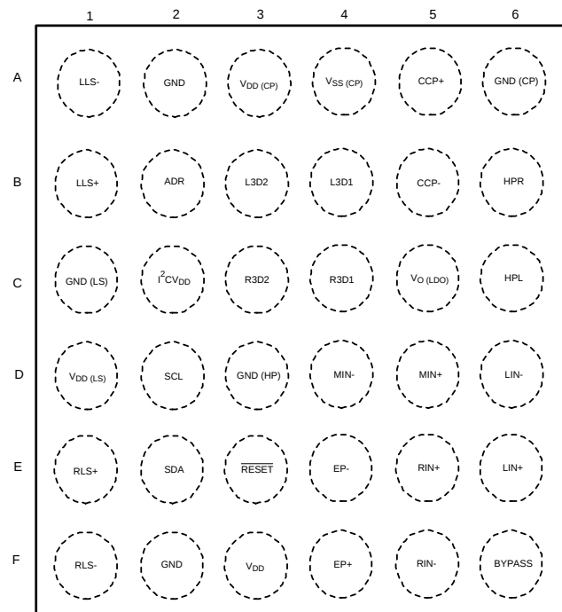
Figure 2. DSBGA Package See Package Number YPG0036CCA
