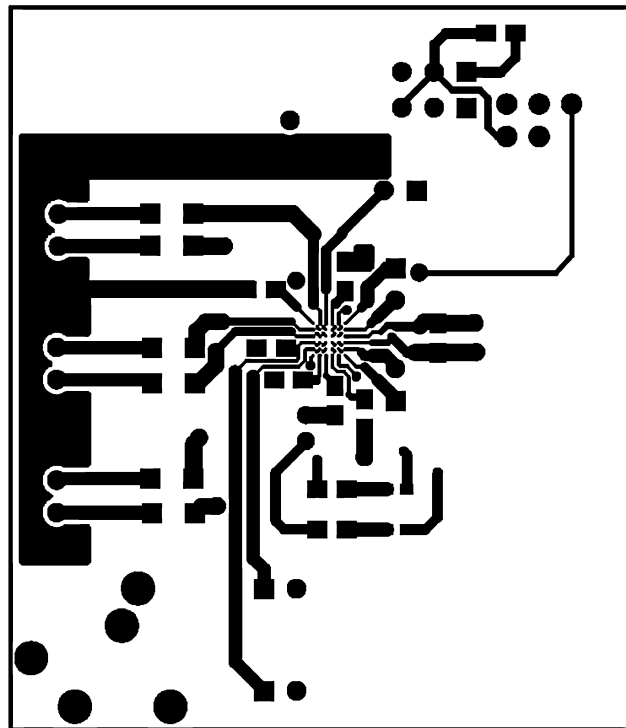
Figure 55. Top Layer
