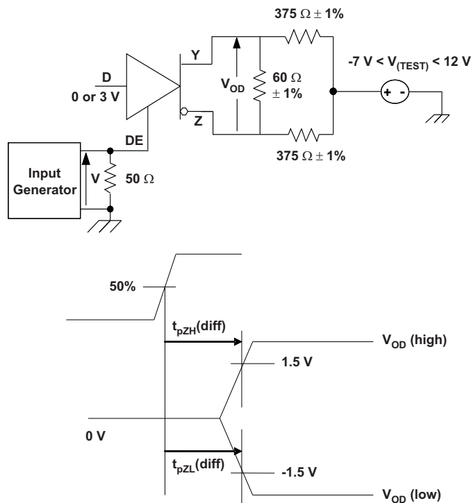
Figure 16. Driver Enable Time From DE to V_{OD}
