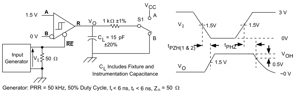
Figure 26. Receiver High-Level Enable and Disable Time Test Circuit and Voltage Waveforms
