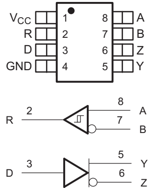
SN65HVD30, SN65HVD31, SN65HVD32, D Package 8-Pin SOIC Top View
