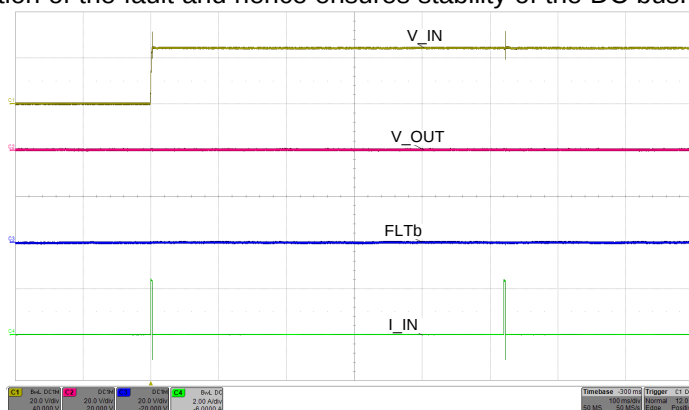
MODE pin connected to RTN VIN = 24 V R_{ILIM} = 5.36 \text{ k}\Omega Figure 45. Start-Up with Short on Output
