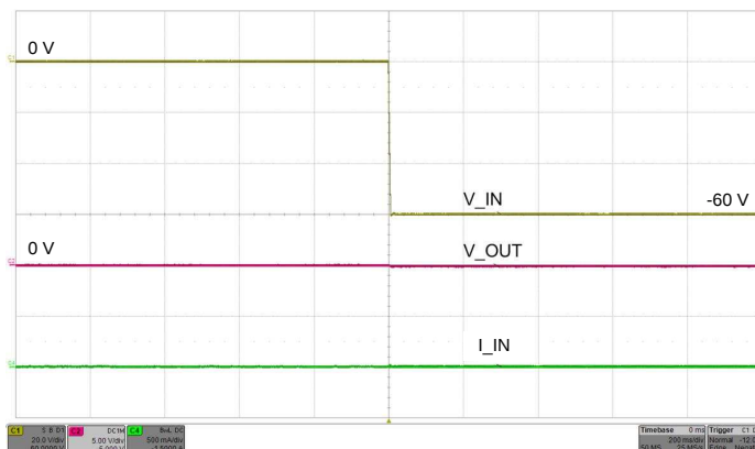
Figure 36. Reverse Input Protection at -60 V
