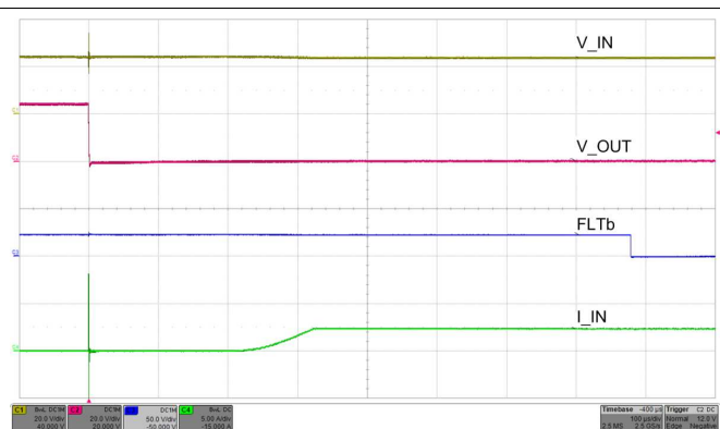
Figure 44. Zoomed at the Instance of Output Short
