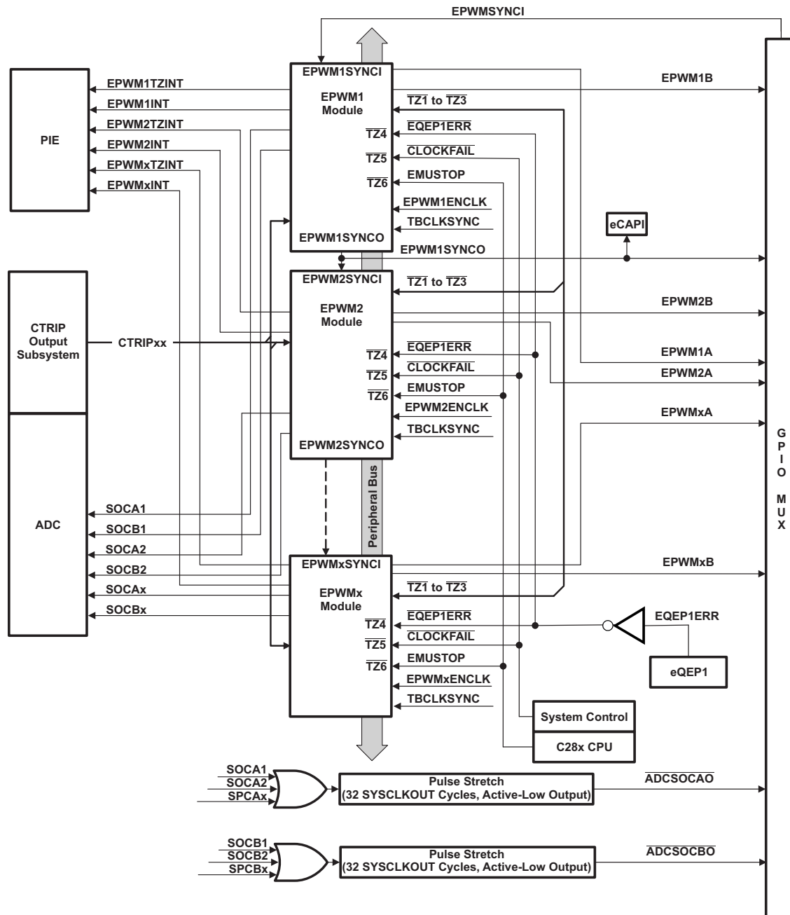
Figure 6-37. ePWM
