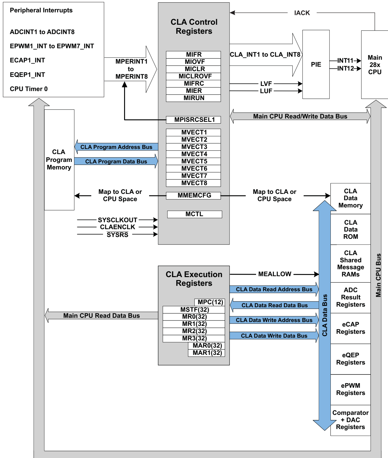
Figure 6-15. CLA Block Diagram
