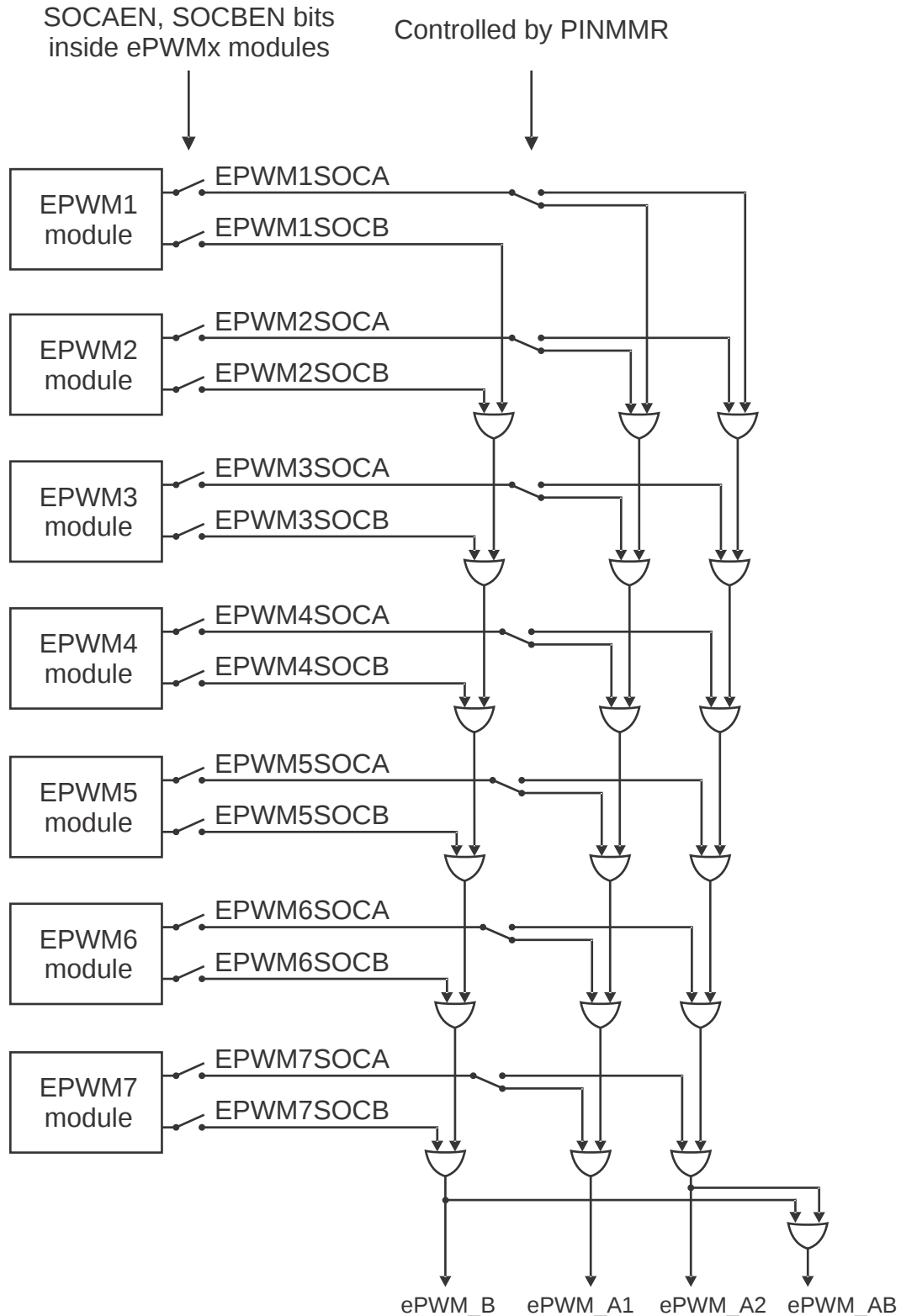
Figure 7-10. ADC Trigger Source Generation from ePWMx
