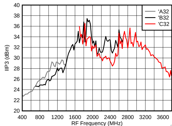
IIP3 Performance Across Frequency
