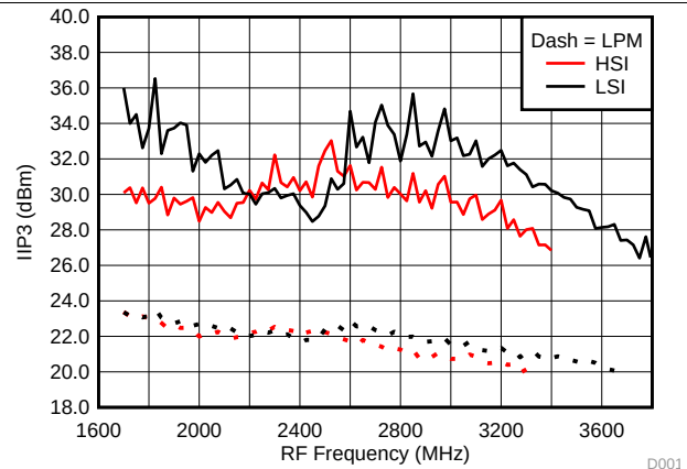
Figure 50. IIP3 vs Frequency over H/LSI, LPM
