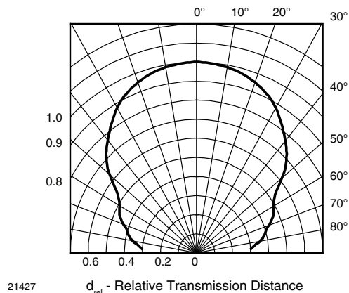
Fig. 11 - Horizontal Directivity
