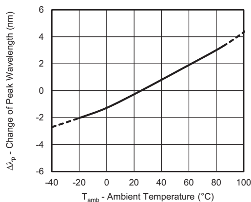
Fig. 7 - Change of Peak Wavelength vs. Ambient Temperature
