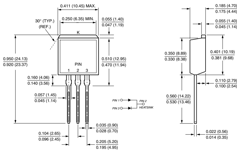
TO-262AA
