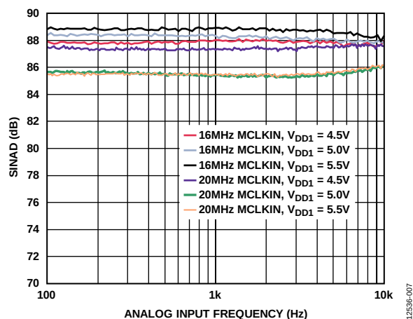
Figure 7. SINAD vs. Analog Input Frequency
