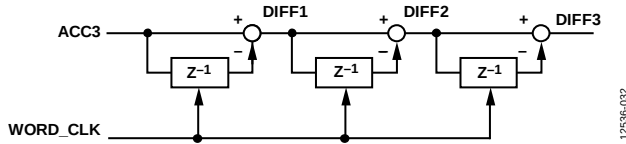
Figure 32. Differentiator
