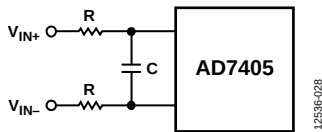
Figure 28. Differential RC Filter Input Network
