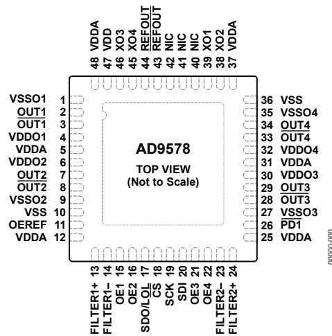
Figure 3. Pin Configuration
