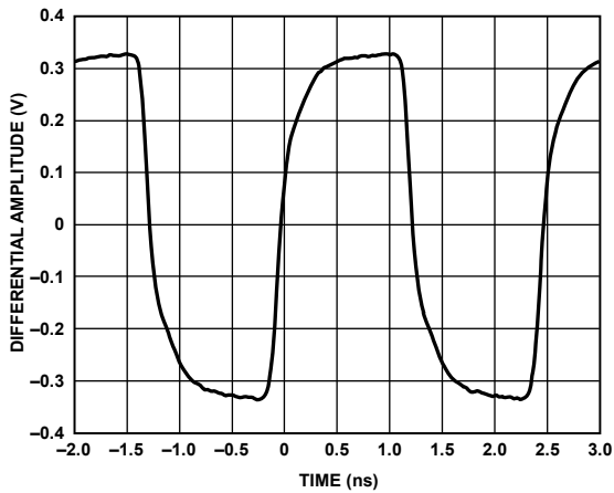
Figure 17. Output Waveform, LVDS (400 MHz)
