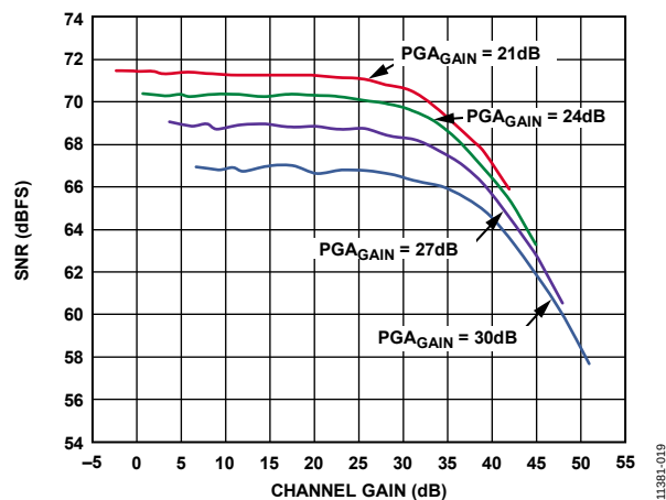
Figure 19. SNR vs. Channel Gain and PGA Gain, A_{\text{IN}} = -45 \text{ dBm}
