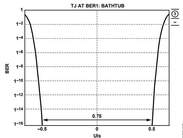
Figure 54. Digital Outputs Bathtub Curve, External 100 \Omega Terminations at 5.0 Gbps
