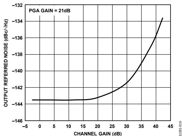
Figure 16. Short-Circuit, Output Referred Noise vs. Channel Gain, LNA Gain = 21.6 dB, PGA Gain = 21 dB, V_{\text{GAIN}} = 1.6 \text{ V}
