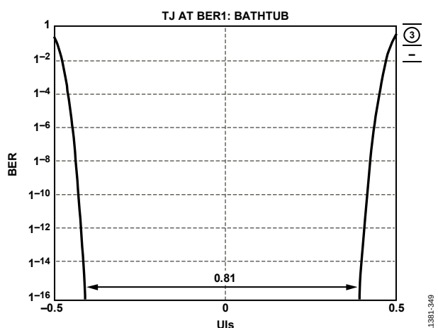
Figure 51. Digital Outputs Bathtub Curve, External 100 \Omega Terminations at 2.5 Gbps
