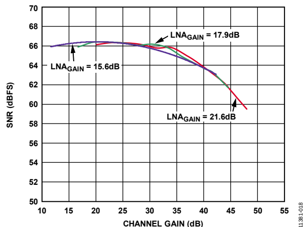
Figure 18. SNR vs. Channel Gain and LNA Gain, A_{\text{OUT}} = -1.0 \text{ dBFS}
