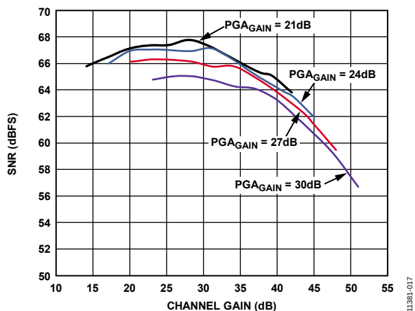
Figure 17. SNR vs. Channel Gain and PGA Gain, A_{\text{OUT}} = -1.0 \text{ dBFS}
