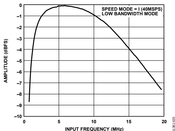
Figure 20. Antialiasing Filter (AAF) Pass-Band Response, LPF Cutoff = 1 \times (1/3) \times f_{\text{SAMPLE}} , HPF = 1/12 \times \text{LPF Cutoff}
