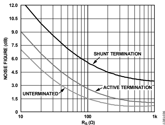
Figure 35. Noise Figure vs. R_S for Shunt Termination, Active Termination Matched and Untermated Inputs, V_{GAIN} = 1.6 \text{ V}
