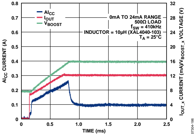
Figure 83. A_{I_{CC}} Current vs. Time for 24 mA Step Through 500 \Omega Load with External 51 k \Omega Compensation Resistor
