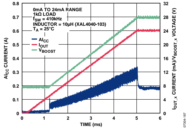
Figure 84. A_{I_{CC}} Current vs. Time for 24 mA Step Through 1 k \Omega Load with Slew Rate Control
