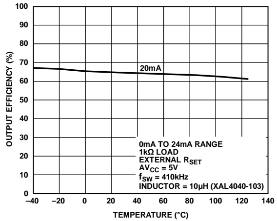
Figure 58. Output Efficiency vs. Temperature (See Figure 79)
