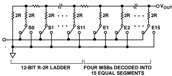
Figure 71. DAC Ladder Structure
