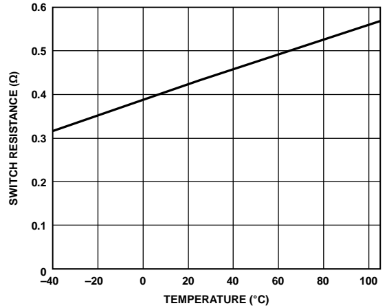
Figure 59. Switch Resistance vs. Temperature
