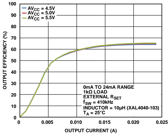
Figure 57. Output Efficiency vs. Output Current (See Figure 79)
