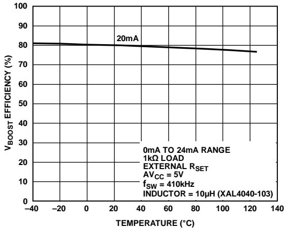
Figure 56. Efficiency at V_{BOOST\_X} vs. Temperature (See Figure 79)
