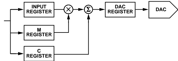
Figure 77. Digital Offset and Gain Control
