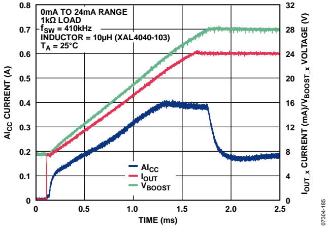
Figure 82. A_{I_{CC}} Current vs. Time for 24 mA Step Through 1 k \Omega Load with External 51 k \Omega Compensation Resistor
