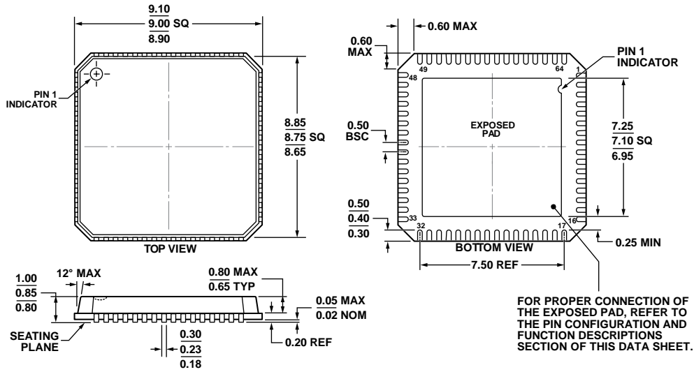
Figure 88. 64-Lead Lead Frame Chip Scale Package [LFCSP_VQ] 9 mm × 9 mm Body, Very Thin Quad (CP-64-3) Dimensions shown in millimeters
