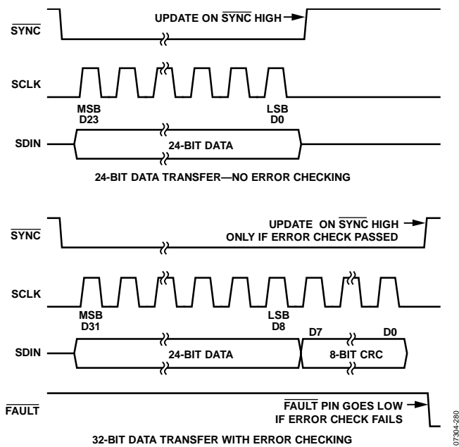
Figure 78. PEC Timing
