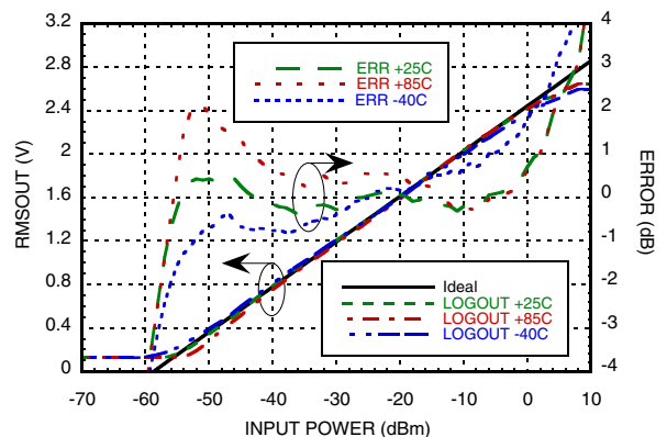
RMSOUT & Error vs. Pin @ 3500 MHz [1][2]
