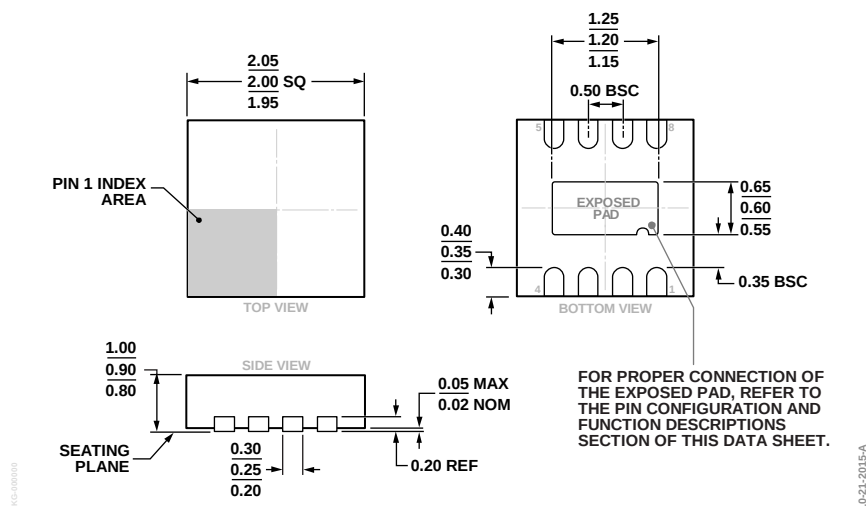
Figure 15. 8-Lead Lead Frame Chip Scale Package [LFCS] 2 mm × 2 mm Body and 0.90 mm Package Height (CP-8-26)
