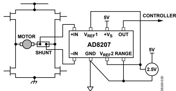
Figure 33. H-Bridge Motor Control Application
