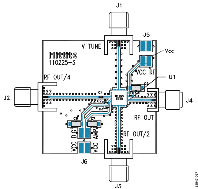
Figure 17. Evaluation PCB
