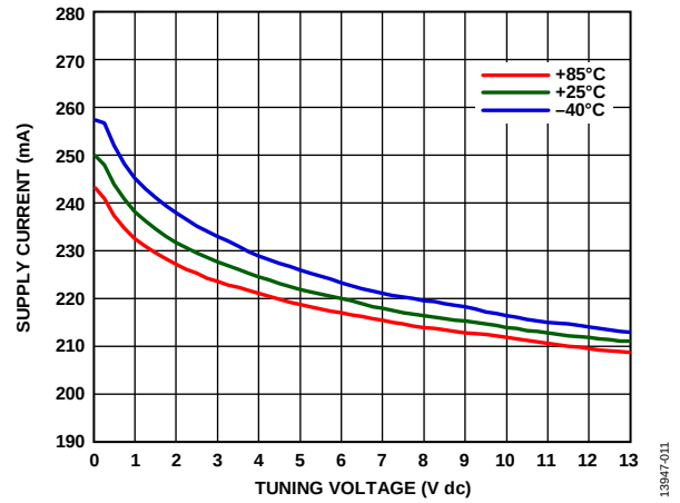
Figure 11. Supply Current ( I_{CC} ) vs. Tuning Voltage
