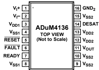
Figure 3. Pin Configuration
