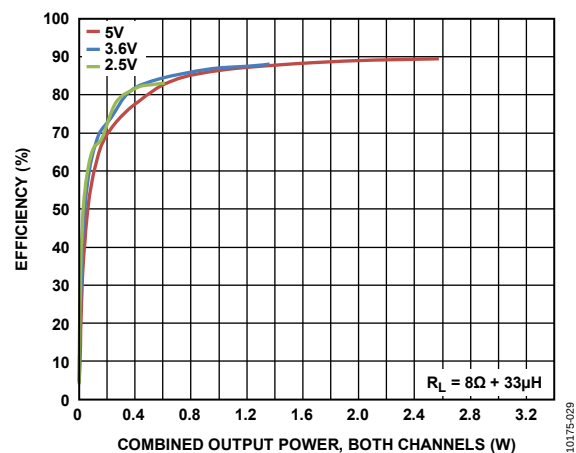
Figure 22. Efficiency vs. Output Power into 8\Omega
