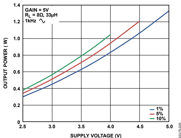
Figure 21. Maximum Output Power vs. Supply Voltage, R_L = 8\Omega
