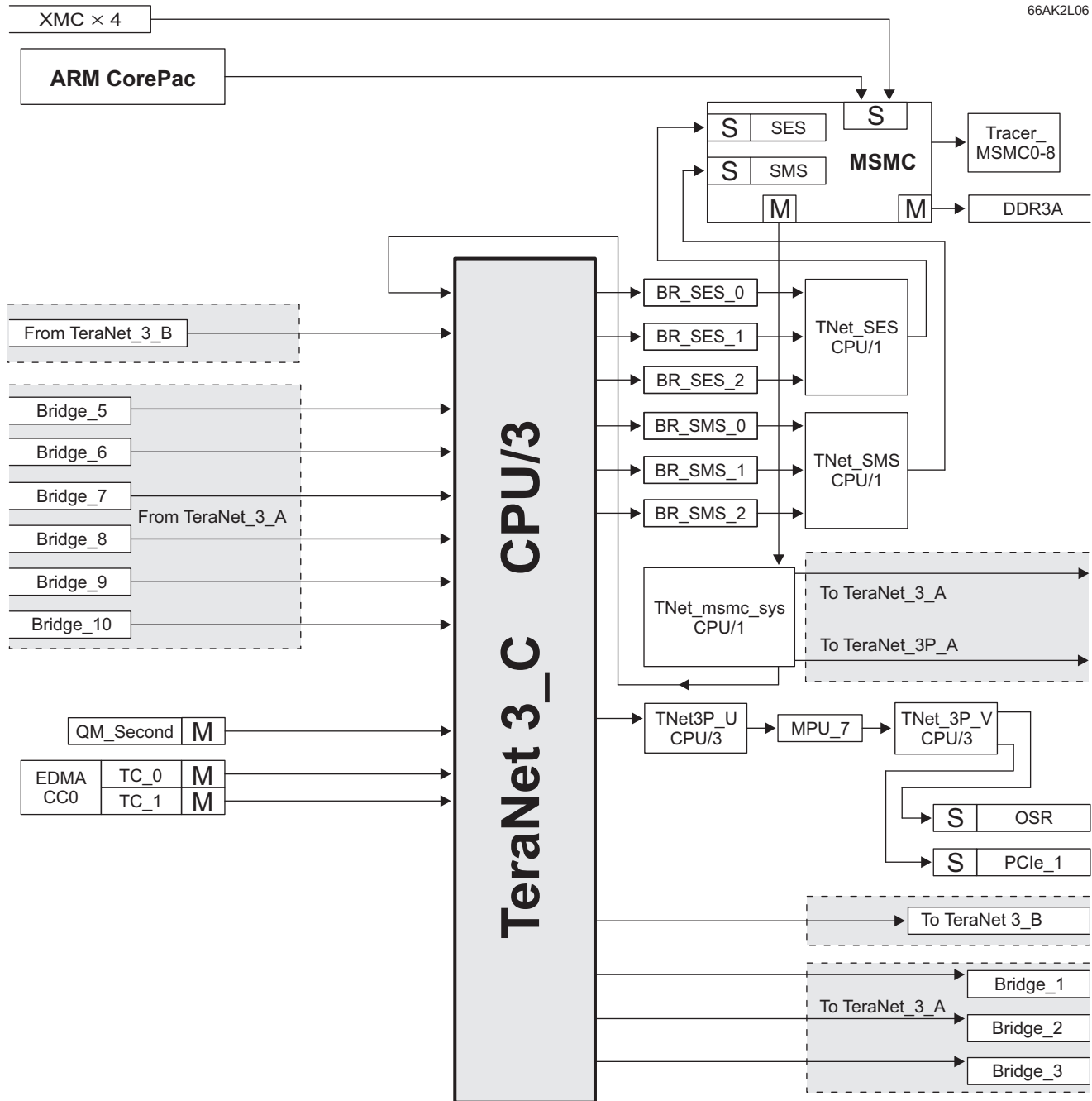
Figure 8-4. TeraNet 3_C
