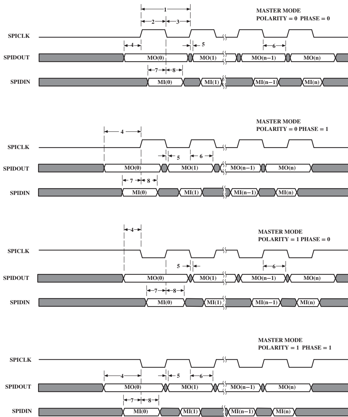
Figure 11-46. SPI Master Mode Timing Diagrams — Base Timings for 3-Pin Mode
