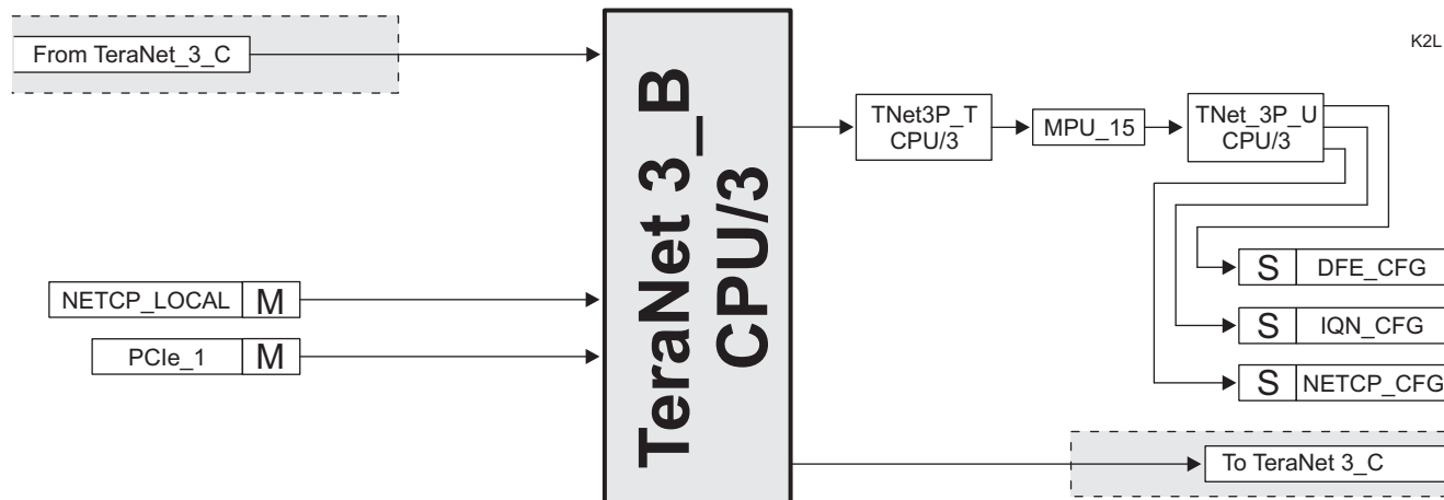
Figure 8-3. TeraNet 3_B
