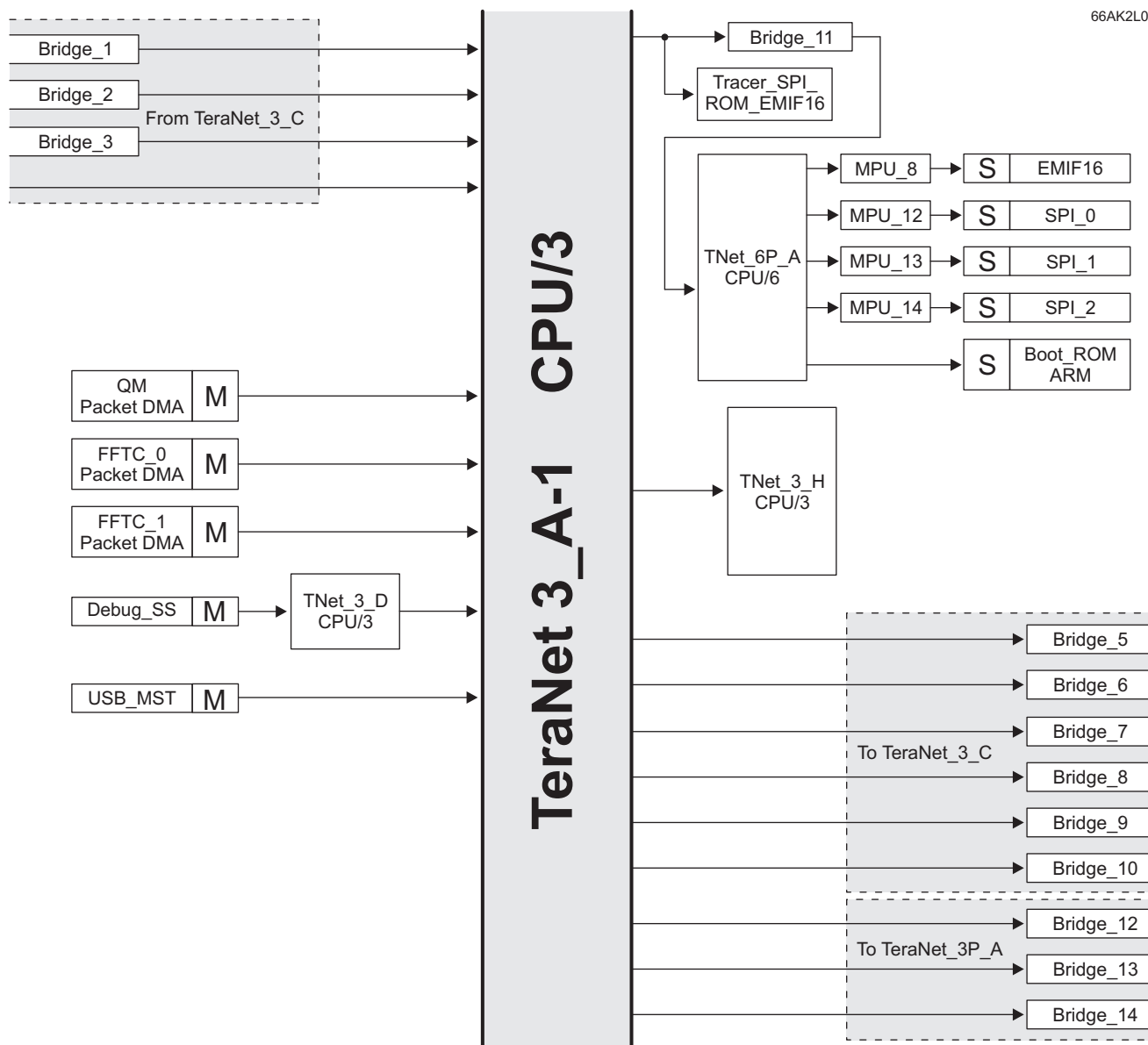
Figure 8-1. TeraNet 3_A-1
