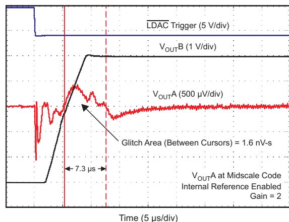
Figure 43. Channel-to-Channel Crosstalk, 5-V Rising Edge
