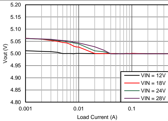
Figure 73. Output Voltage Regulation
