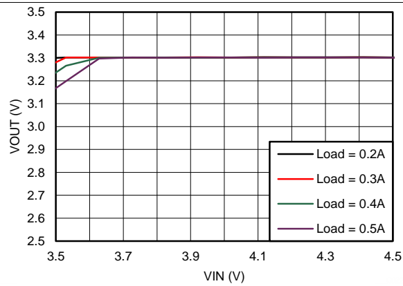
Figure 13. Drop-Out Curve
