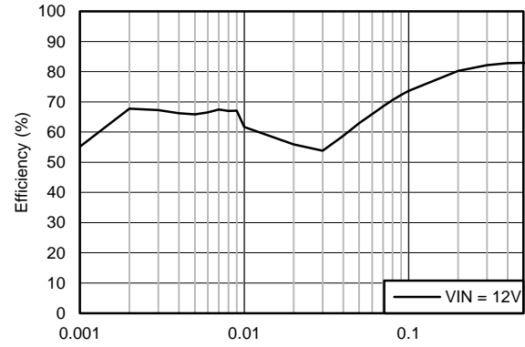
Figure 78. Efficiency
