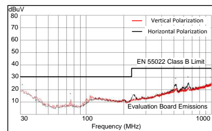
Radiated Emission Graph V_{IN} = 12\text{ V} , V_{OUT} = 3.3\text{ V} , F_S = 500\text{ kHz} , I_{OUT} = 0.5\text{ A}
