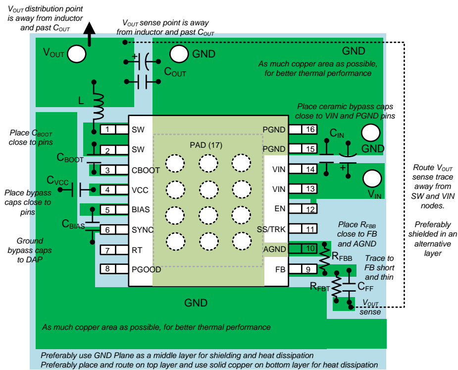
Figure 108. LM43600-Q1 PCB Layout Example
