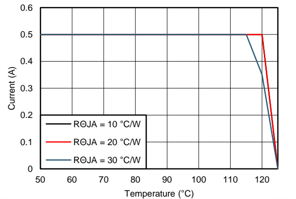
Figure 70. Derating Curve
