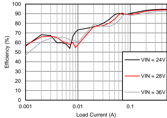
Figure 84. Efficiency
