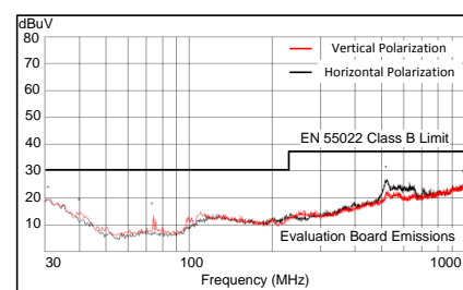
Radiated Emission Graph V_{IN} = 12 \text{ V} , V_{OUT} = 3.3 \text{ V} , F_S = 500 \text{ kHz} , I_{OUT} = 1 \text{ A}
