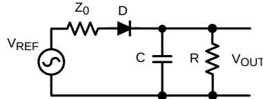
Figure 50. Diode Detector
