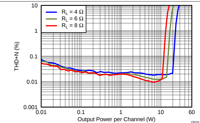
Figure 19. THD+N vs Output Power
