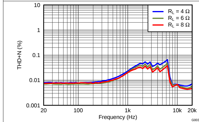
Figure 16. THD+N vs Frequency
