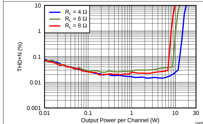
Figure 18. THD+N vs Output Power
