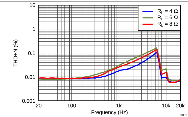
Figure 15. THD+N vs Frequency
