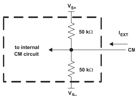
Figure 83. CM Input Circuit
