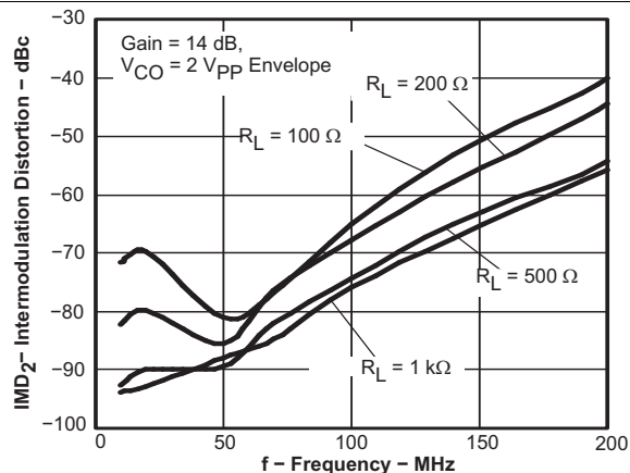
Figure 17. IMD2 vs Frequency
