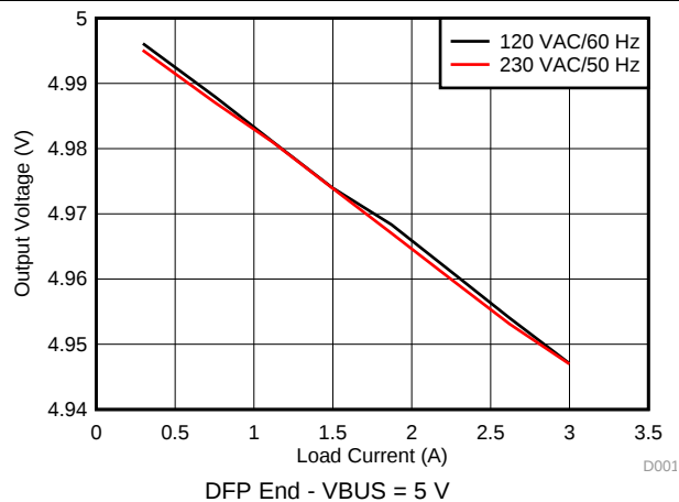
Figure 46. Load Regulation
