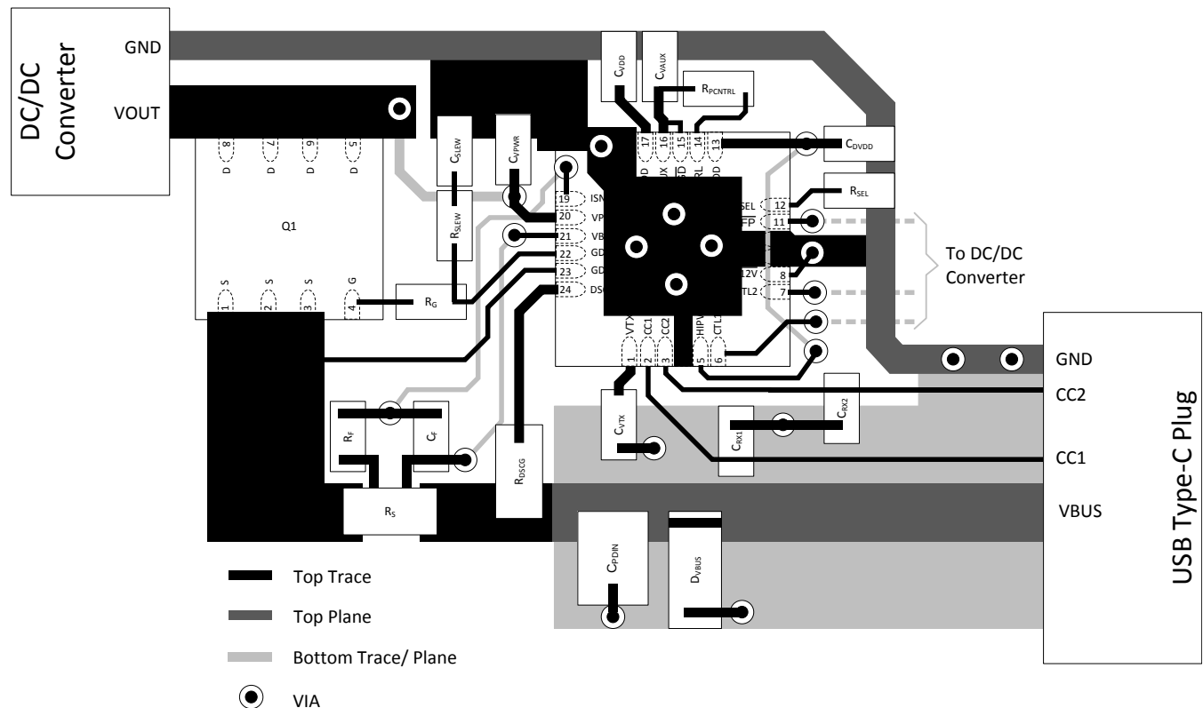
Figure 68. Example Layout
