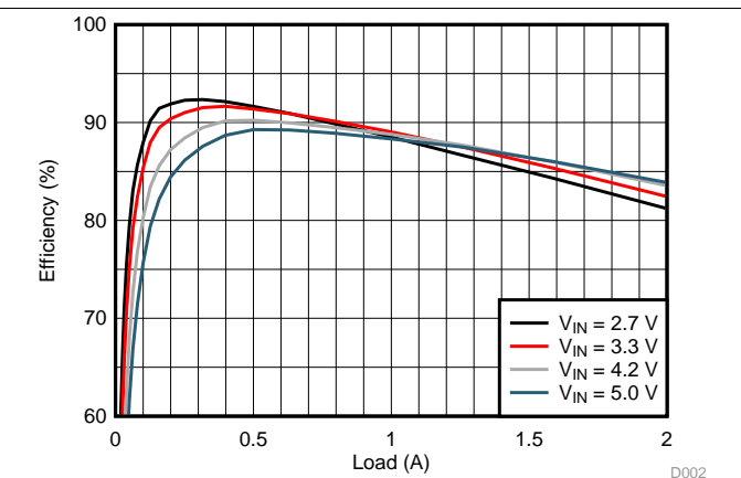
Figure 8. Efficiency, Forced PWM Mode (2.0MHz)
