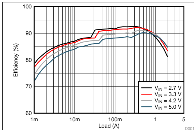
Figure 7. Efficiency, PWM/PSM Mode (2.0 MHz)
