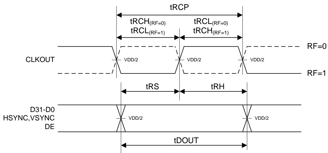
Figure 20. LVC MOS Output Switching Timing Diagrams
