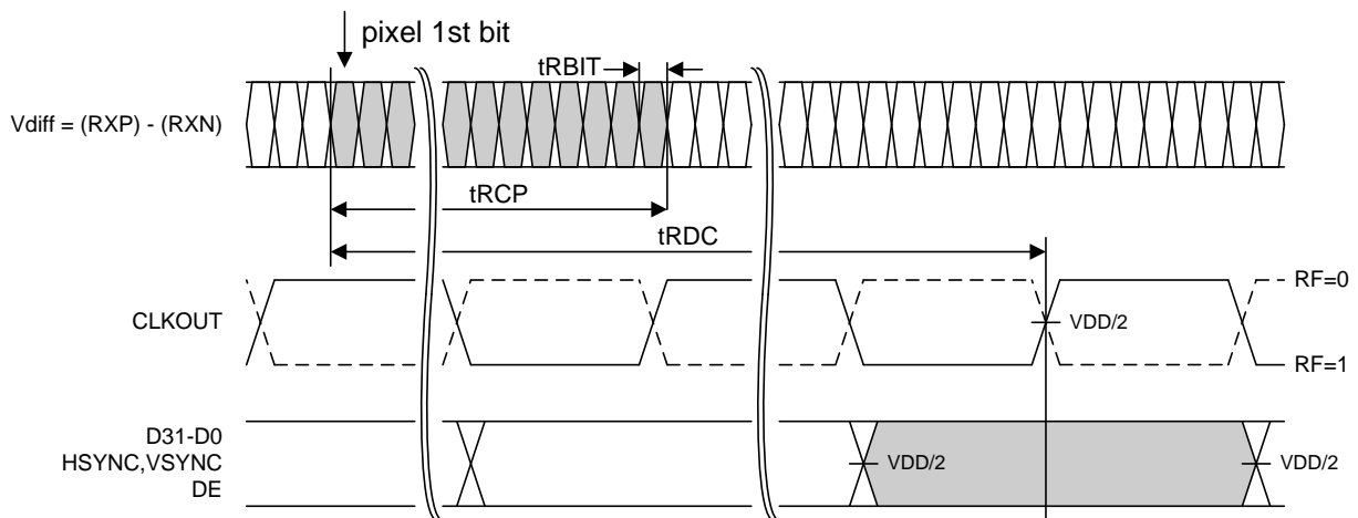
Figure 26. THCV236-Q Latency
