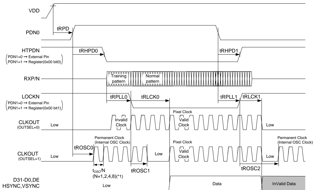
Figure 28. THCv236-Q Lock/Unlock Sequence
