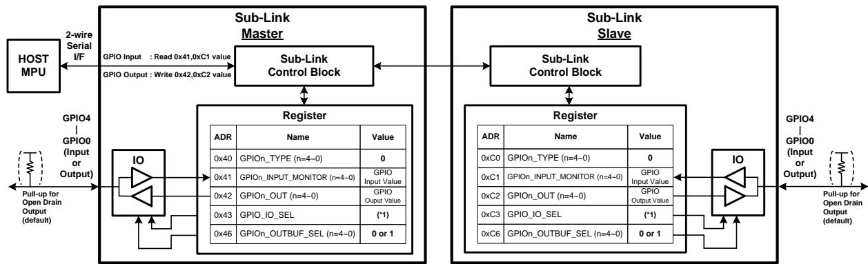
Figure 15. Programmable GPIO
