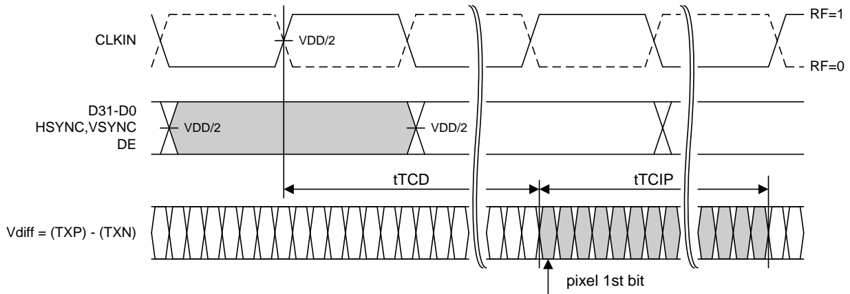
Figure 25. THCV235-Q Latency
