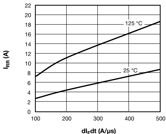
Fig. 15 - Typical D5 - D6 Clamping Diode Reverse Recovery Current vs. dI_F/dt , V_R = 200 V, I_F = 50 A
