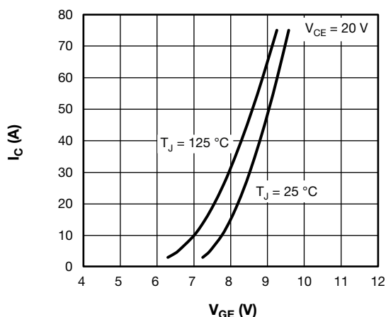
Fig. 4 - Typical Q1 - Q4 Trench IGBT Transfer Characteristics V_{CE} = 20\text{ V}
