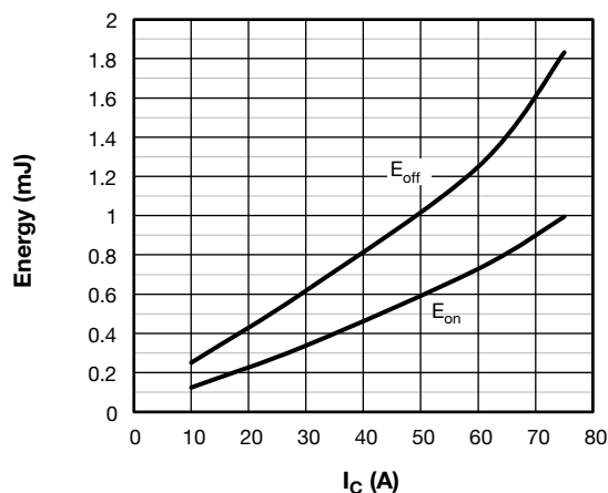
Fig. 25 - Typical Q2 - Q3 Trench IGBT Energy Loss vs. I_C (with Freewheeling External TO-247 Diode Discrete 30ETH06), T_J = 125^\circ\text{C} , V_{CC} = 300\text{ V} , R_g = 4.7\ \Omega , V_{GE} = 15\text{ V} , L = 500\ \mu\text{H}
