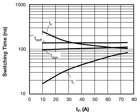
Fig. 26 - Typical Q2 - Q3 Trench IGBT Switching Time vs. I_C (with Freewheeling External TO-247 Diode Discrete 30ETH06), T_J = 125^\circ\text{C} , V_{CC} = 300\text{ V} , R_g = 4.7\ \Omega , V_{GE} = 15\text{ V} , L = 500\ \mu\text{H}
