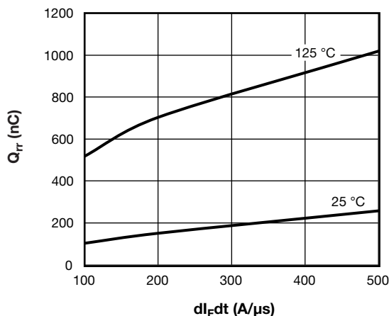
Fig. 16 - Typical D5 - D6 Clamping Diode Reverse Recovery Charge vs. dI_F/dt , V_R = 200 V, I_F = 50 A
