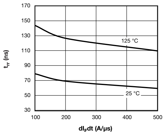
Fig. 14 - Typical D5 - D6 Clamping Diode Reverse Recovery Time vs. dI_F/dt , V_R = 200 V, I_F = 50 A
