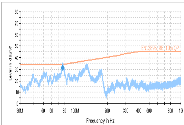
Figure 14: test result(Vertical)
