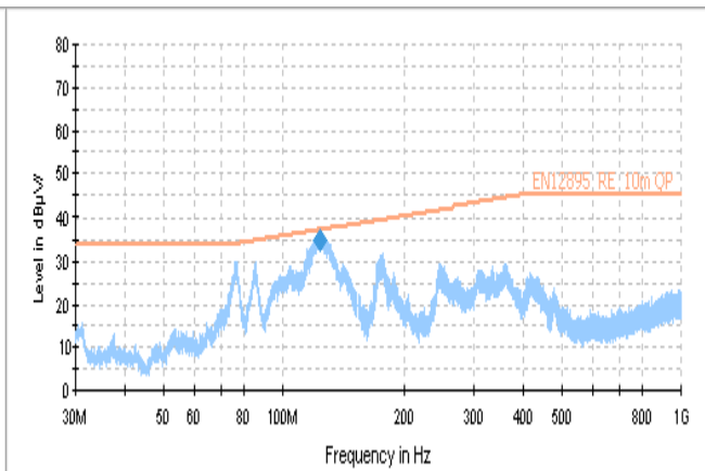
Figure 15: test result(Horizontal)
