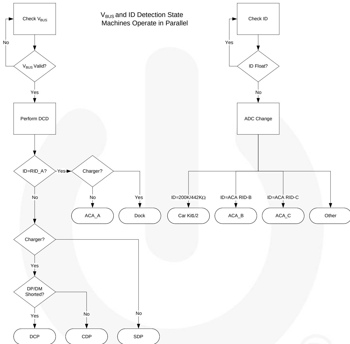
Figure 5. Accessory Discovery State Machine Flow Diagram
