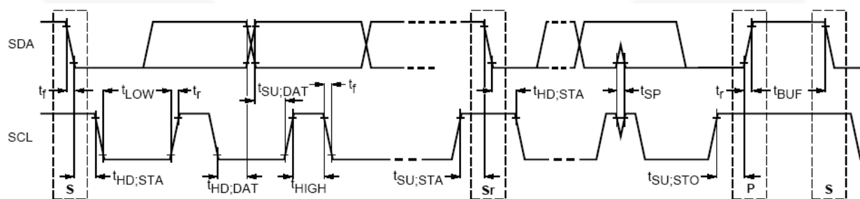
Figure 6. Definition of Timing for Full-Speed Mode Devices on the I 2 C Bus ®
