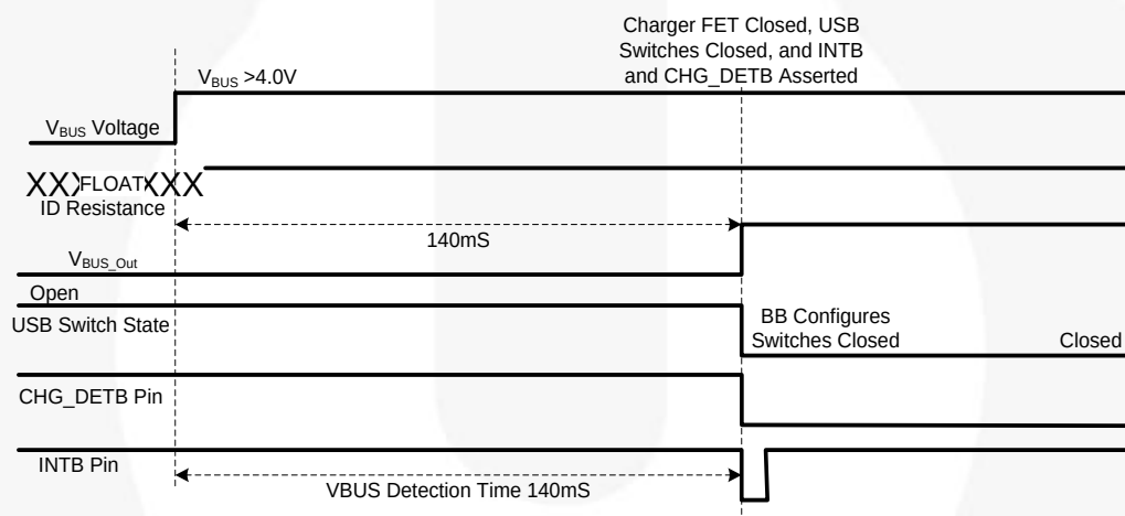
Figure 11. Car Kit Type-1 and Type-2 Attach Timing
