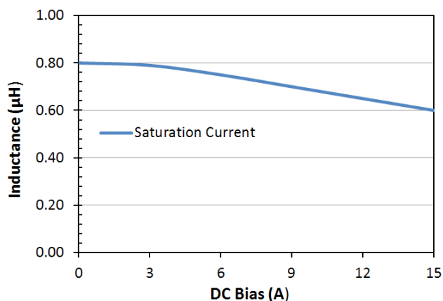
Saturation Current: LPM0530HIR82ME
