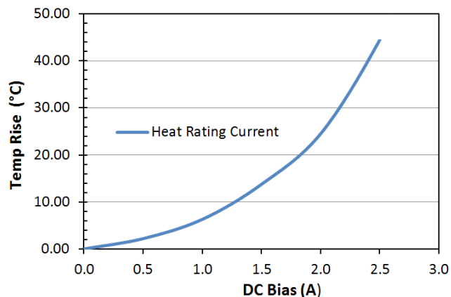
Heat Rating Current: LPM0520HI100ME
