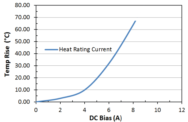
Heat Rating Current: LPM0530HI2R2ME
