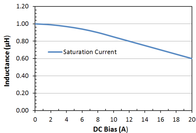
Saturation Current: LPM0630LR1R0ME
