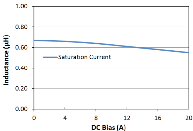
Saturation Current: LPM0530HIR60ME
