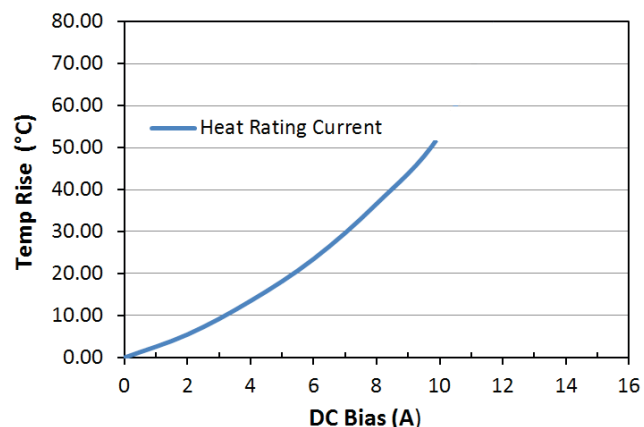
Heat Rating Current: LPM0530HI1R2ME
