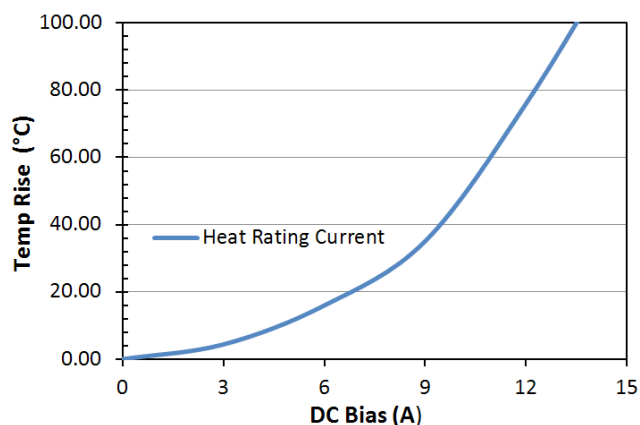
Heat Rating Current: LPM0530HIR82ME
