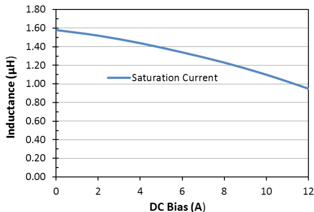
Saturation Current: LPM0530LR1R5ME
