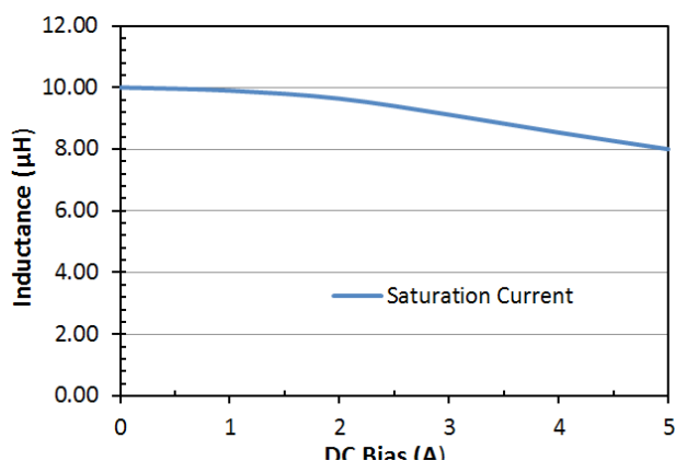
Saturation Current: LPM0520HI100ME
