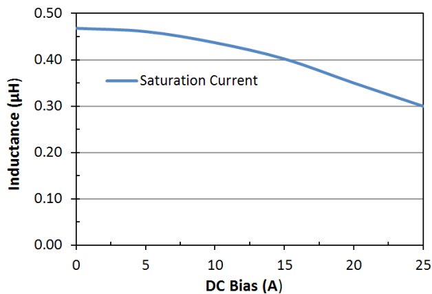
Saturation Current: LPM0630LRR47ME
