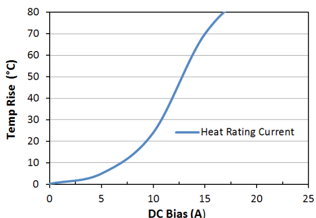
Heat Rating Current: LPM0630HI1R5ME
