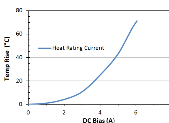
Heat Rating Current: LPM0630HI100ME
