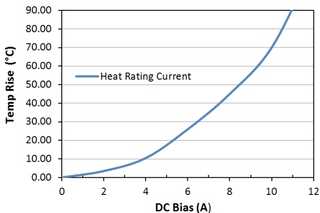
Heat Rating Current: LPM0520LR1R0ME
