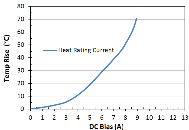
Heat Rating Current: LPM0630LR3R3ME
