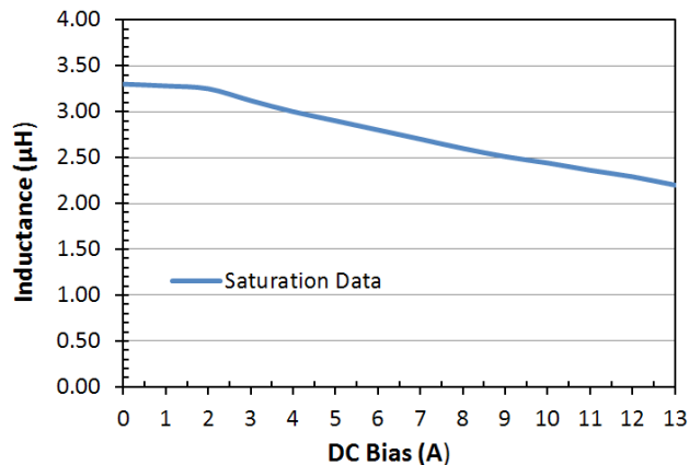
Saturation Current: LPM0630LR3R3ME
