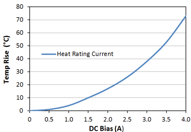
Heat Rating Current: LPM0630HI1R0ME
