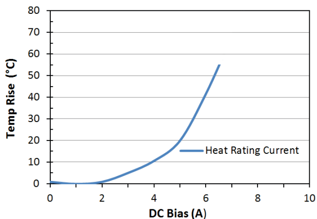
Heat Rating Current: LPM0630HI8R2ME
