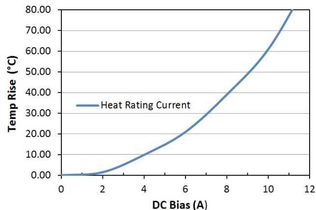
Heat Rating Current: LPM0530HI1R0ME
