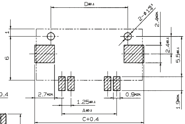
MOUNTING LAYOUT
