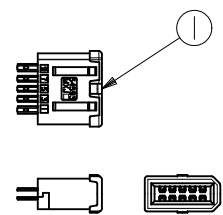
HOUSING ASS'Y
