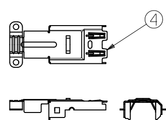
SHELL COVER
