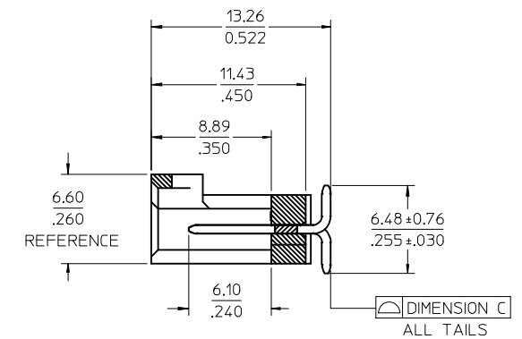
SECTION Z-Z
