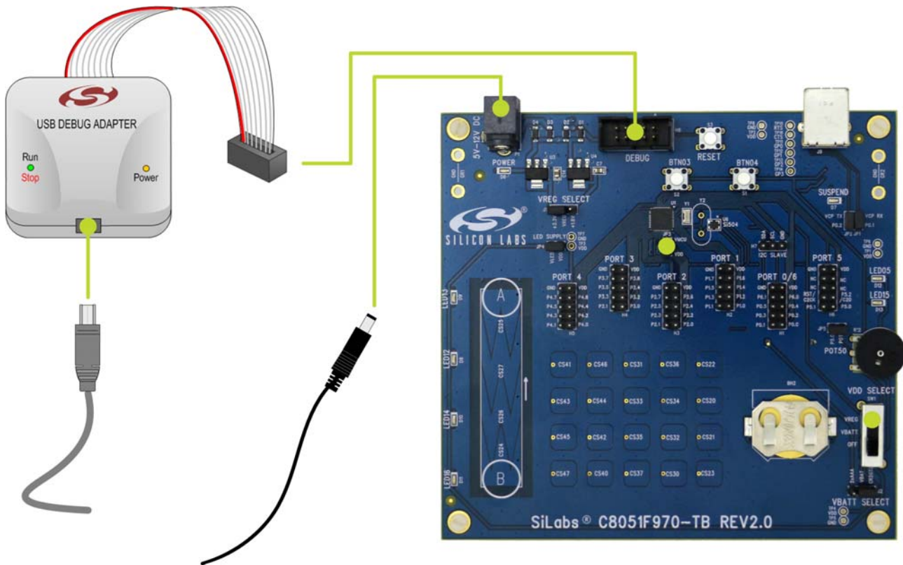
Figure 2. Hardware Setup
