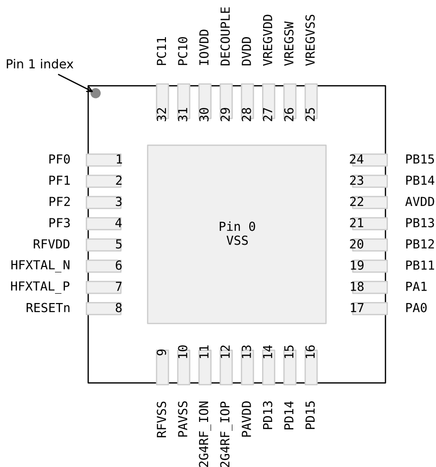
Figure 6.3. EFR32MG1 QFN32 2.4 GHz Pinout
