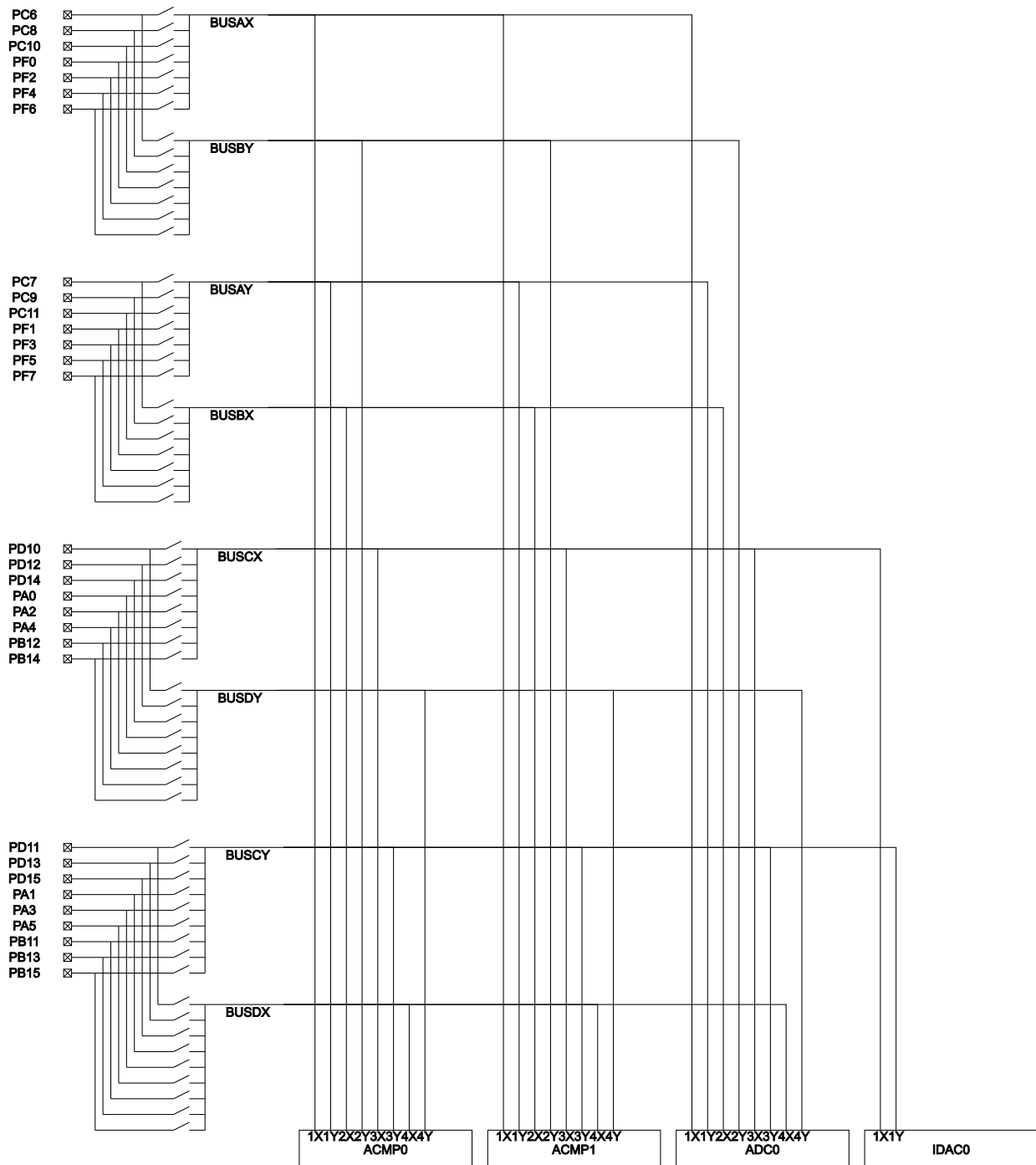
Figure 6.4. EFR32MG1 APORT
