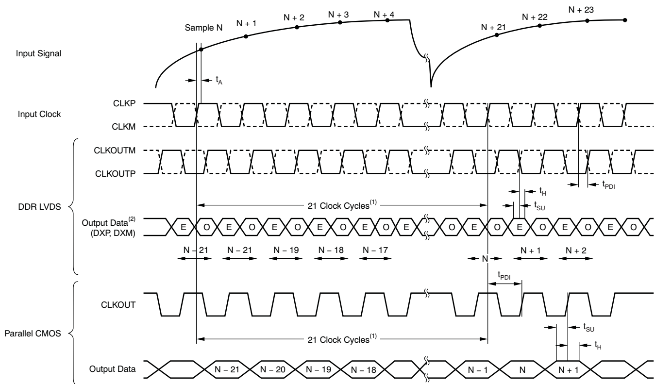
Figure 5. Latency Diagram
