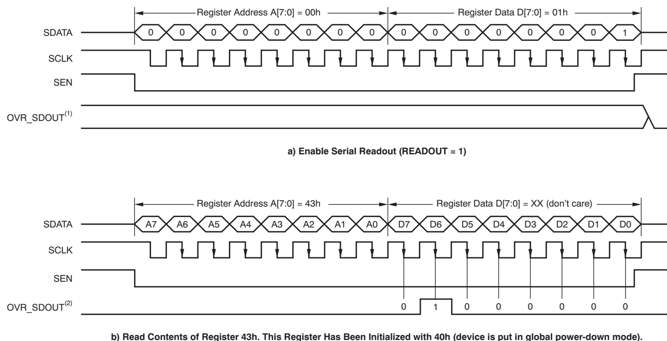
Figure 10. Serial Readout Timing Diagram
