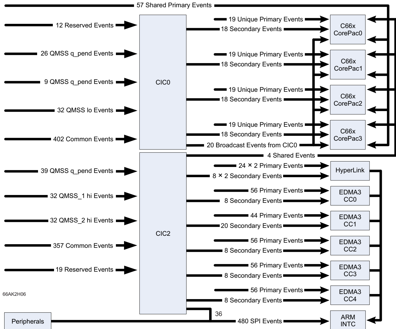
Figure 6-5 66AK2H06 Interrupt Topology
