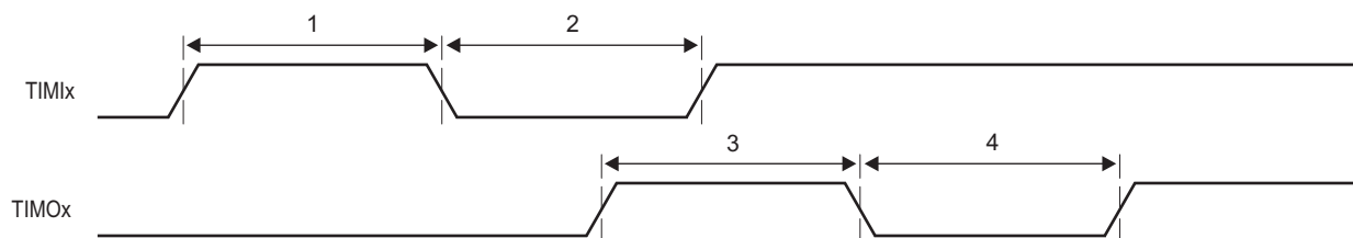
Figure 10-51 Timer Timing
