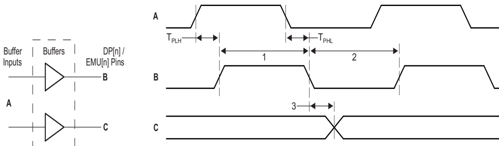
Figure 10-57 Trace Timing
