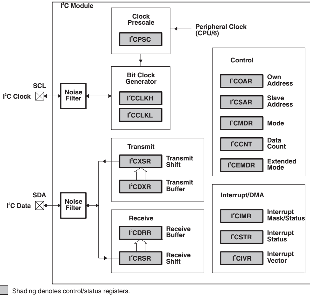
Figure 10-34 I 2 C Module Block Diagram
