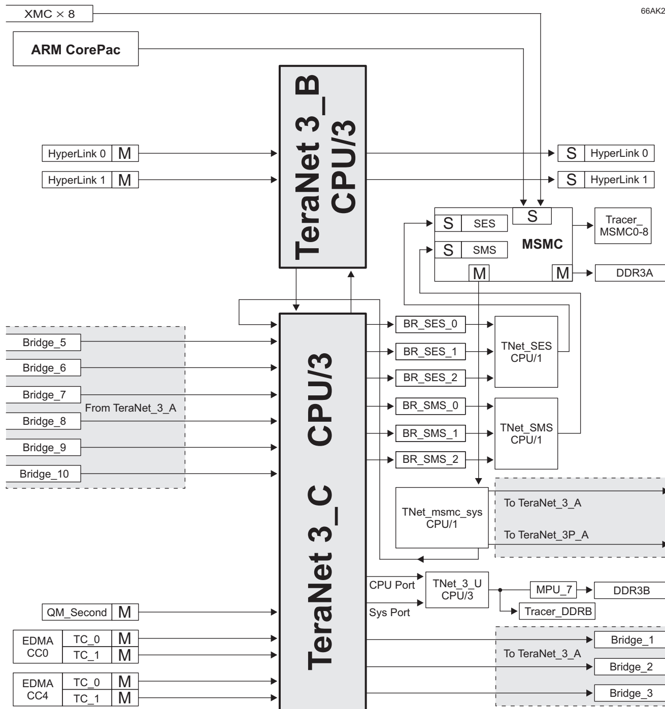
Figure 7-3 TeraNet 3_C
