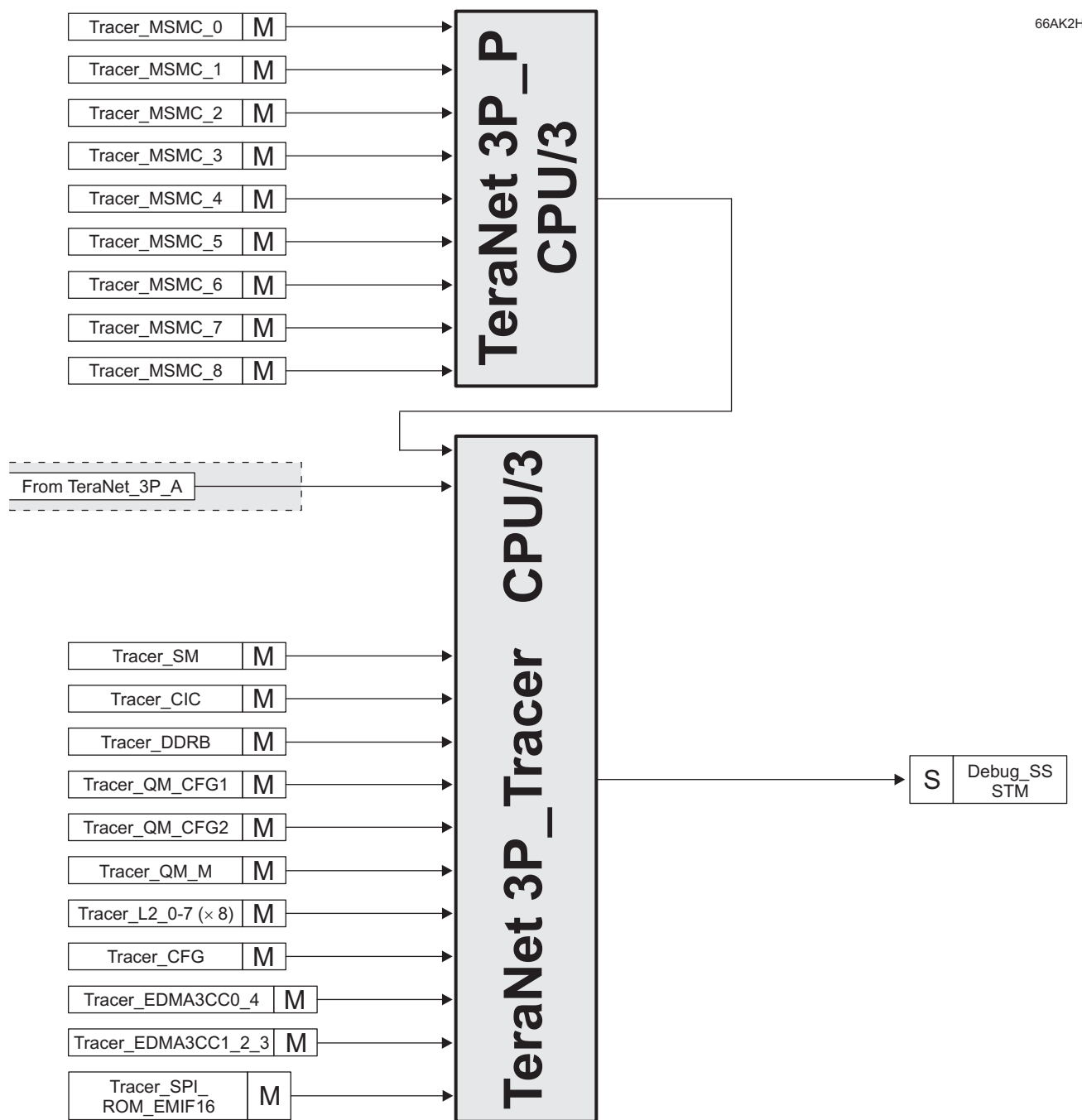
Figure 7-8 TeraNet 3P_Tracer
