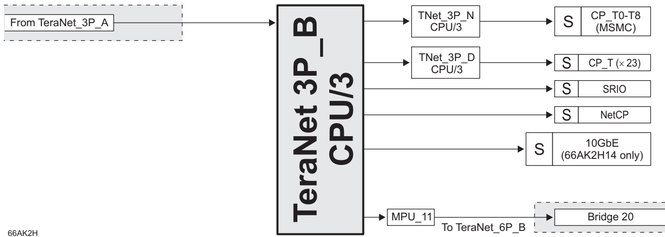
Figure 7-6 TeraNet 3P_B
