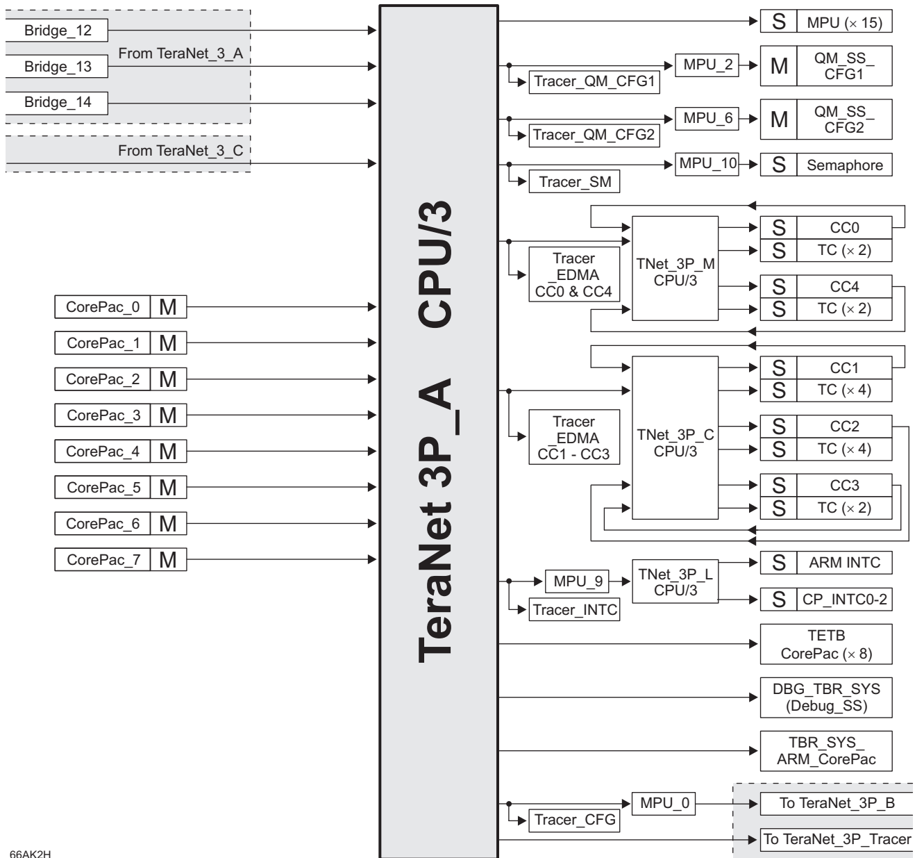
Figure 7-5 TeraNet 3P_A
