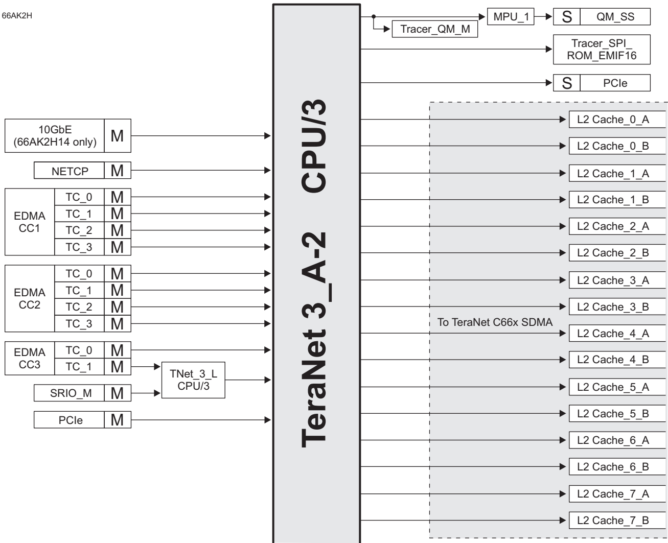
Figure 7-2 TeraNet 3_A-2
