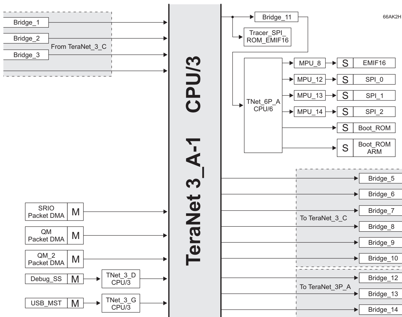
Figure 7-1 TeraNet 3_A-1
