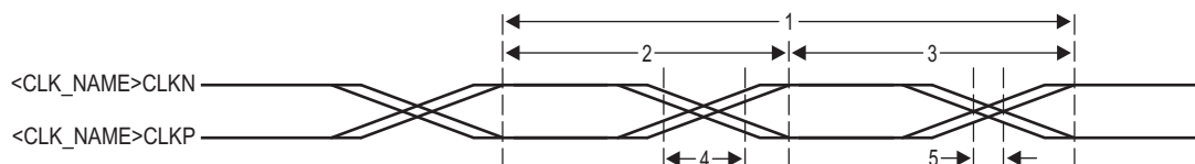
Figure 10-21 Main PLL Controller/SRIO/HyperLink/PCIe/USB Clock Input Timing
